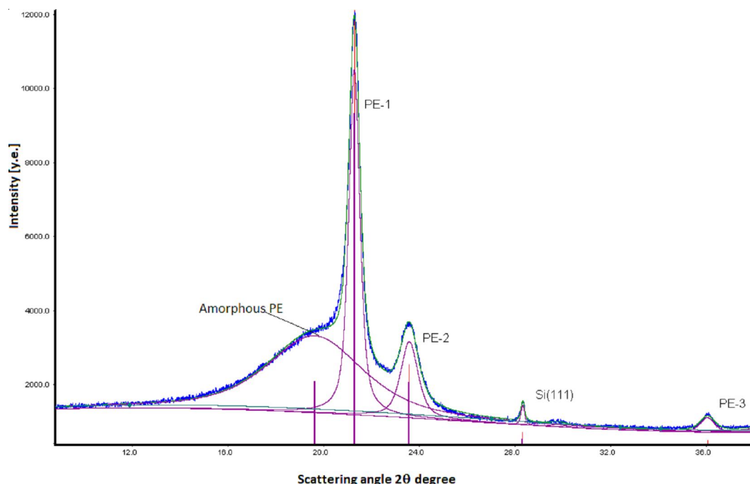
Fig. 4. Diffractogram decomposition on separate peaks and a background by means of approximation of a full profile by analytical functions on an example of the data from sample PE + 1 % nc-Si-36 (Fig. 3).
