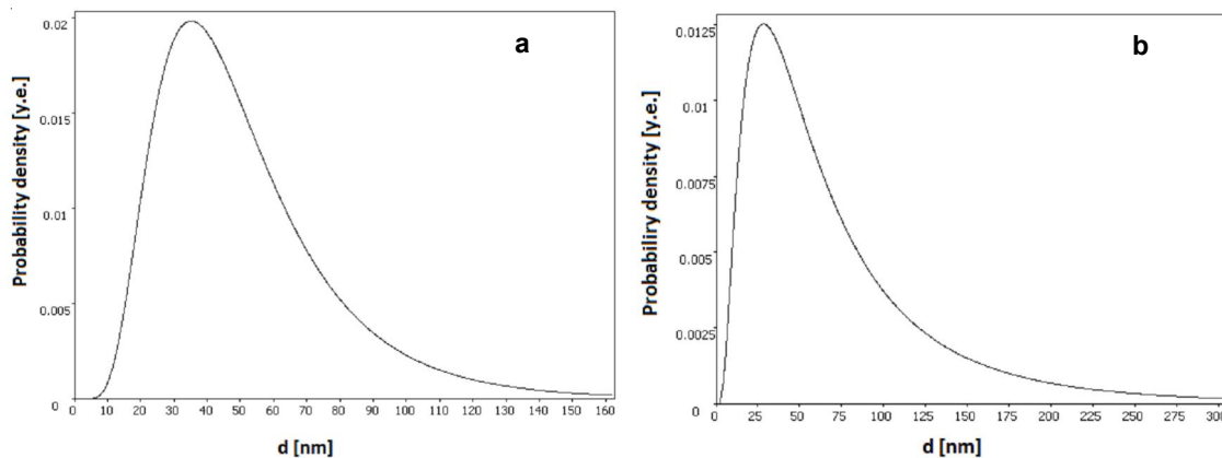
Fig. 2. Density function of particle size in powders nc-Si, received from X-ray diffractogram by means of program PM2K:
