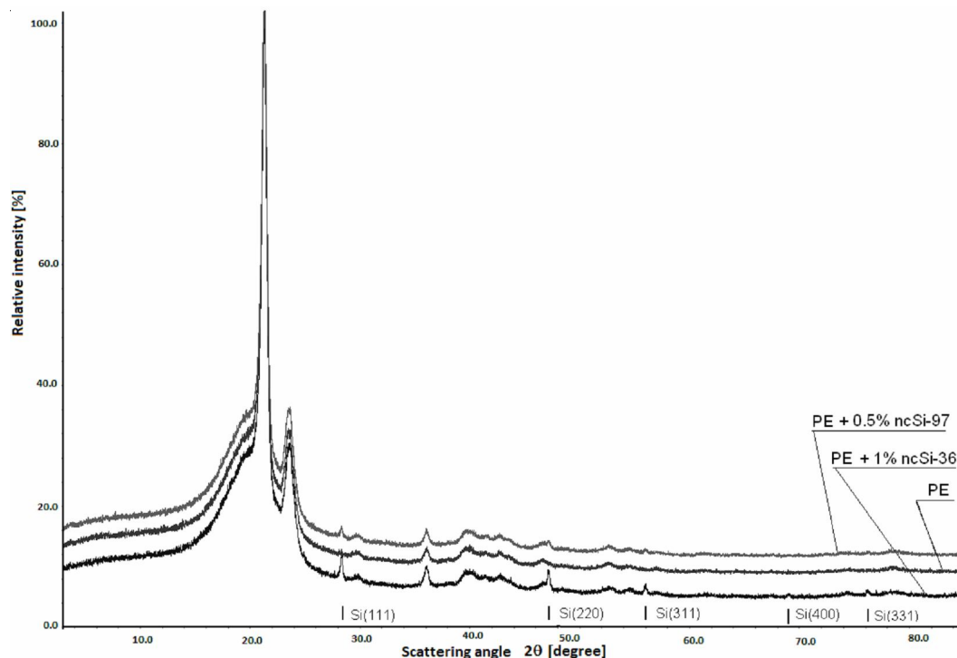
Fig. 3. Diffractograms of the investigated composite films in comparison with diffractogram of pure polyethylene. Below vertical strokes specify reference positions of diffraction lines of silicon with their interference indexes (hkl)
